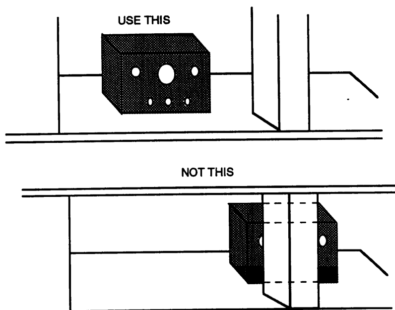
FIGURE 41. Component placement.
