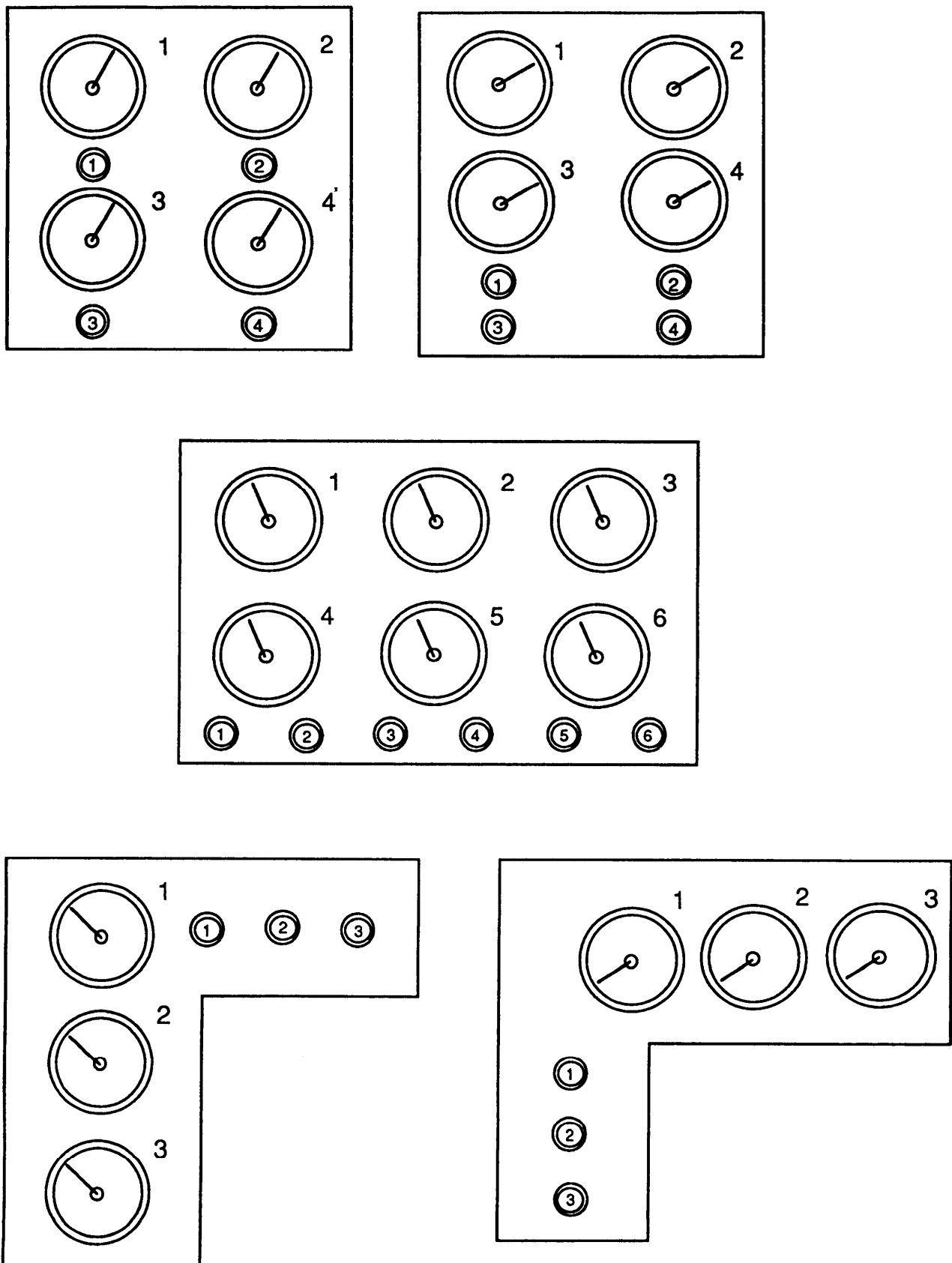
FIGURE 1. Control-display relationship.
