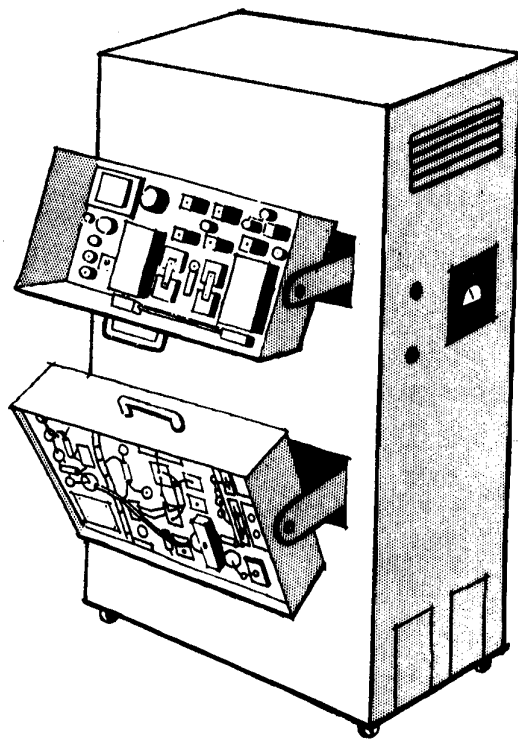
FIGURE 67. Test points on replaceable units.
